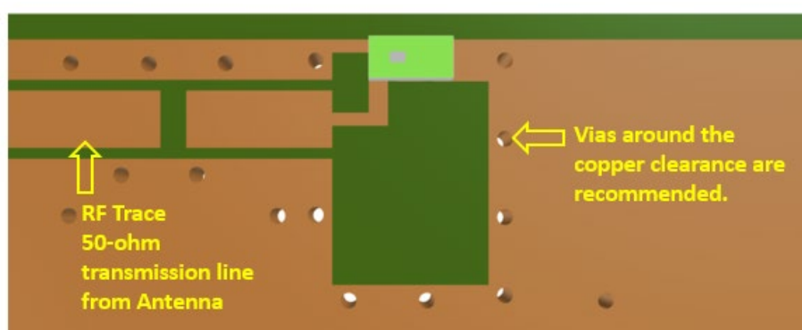
WLA.04 antenna mounted on a PCB, showing transmission line and integration notes.
