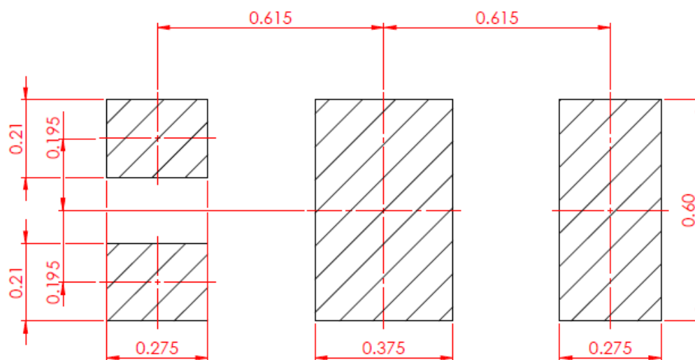
TOP SOLDER PASTE
